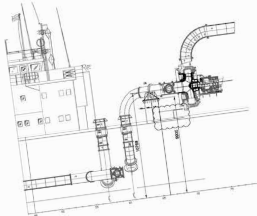
SITUATION 2 Cross Section
