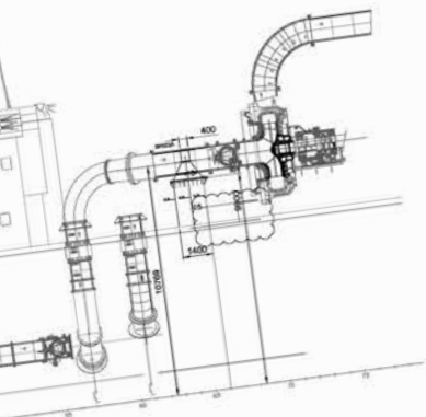
SITUATION 1 Longitudinal Section
